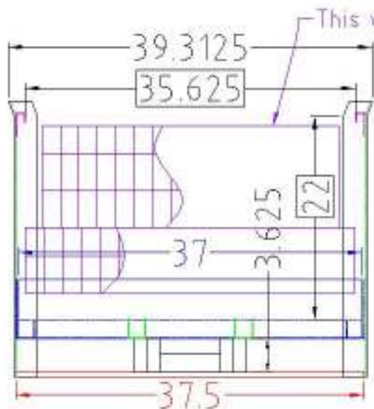
FRONT/BACK ELEVATION
